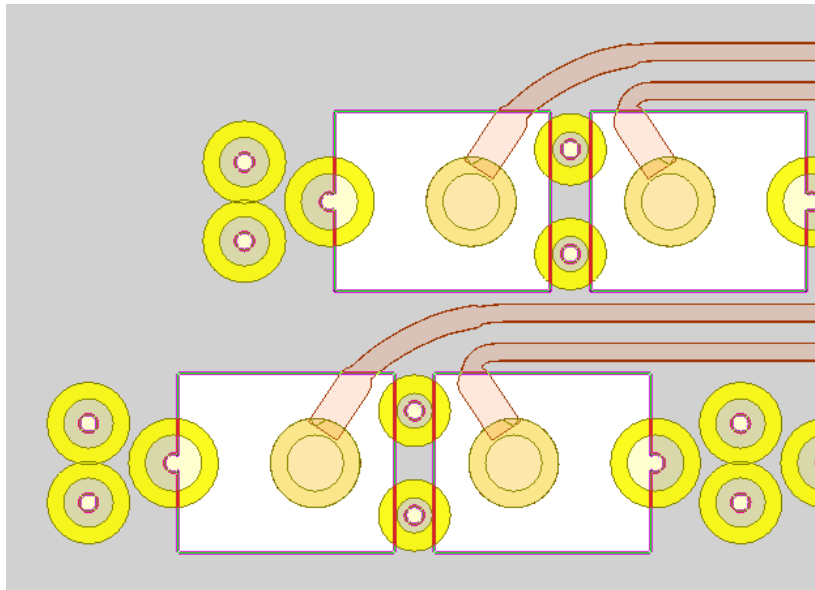
Figure 16: Example X2® Daughtercard Typical High Speed Differential antipad design
